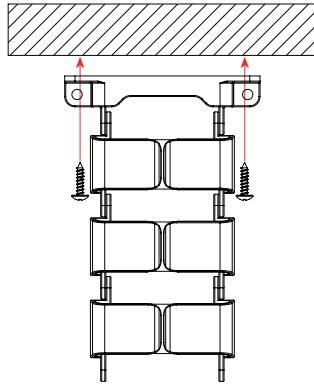
Under worktop mounting
