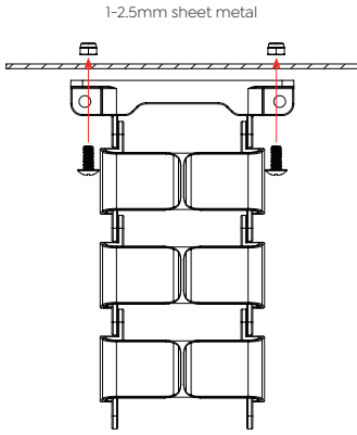
Cable tray mounting
