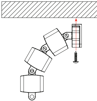
Under worktop mounting
